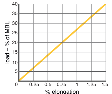
BOB® 12 Strand Elongation (%)
