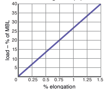
D/V Composite Double Braid Elongation (%)
